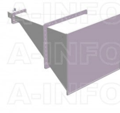
LB-340-20-C-SFSPO Standard Gain Horn Antenna 2.2-3.3GHz 20dB Gain SMA Female
