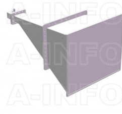
LB-340-20-C-NFSPO Standard Gain Horn Antenna 2.2-3.3GHz 20dB Gain N Type Female
